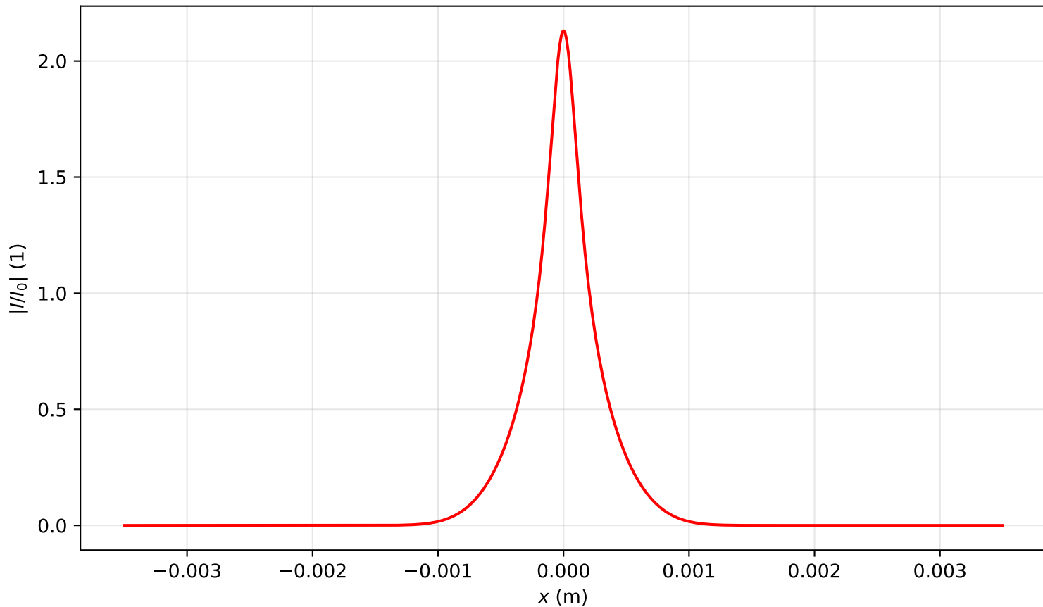
Intensity profile I(x, y = 0, z = 0.239)/I_0 , P_{in}=8.5P_{cr} , artificial time
